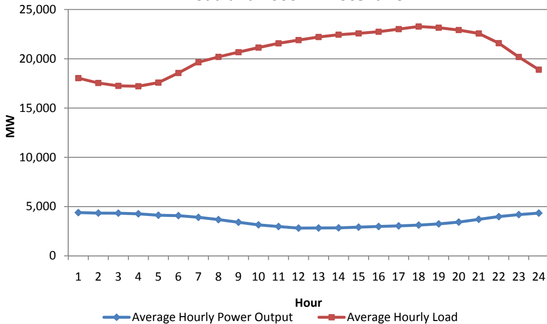
Figure 39. 2007 Mean Diurnal Coincidence for TVA and 7000 MW Wind Scenario
