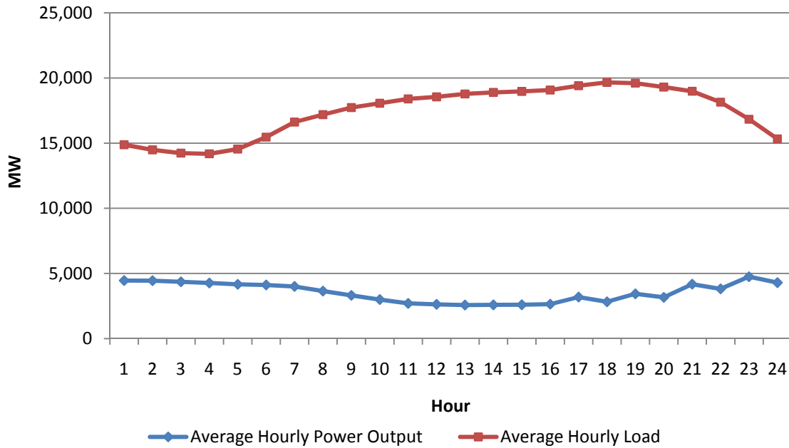
Figure 30. 1998 Mean Diurnal Coincidence for TVA and 7000 MW Wind Scenario
