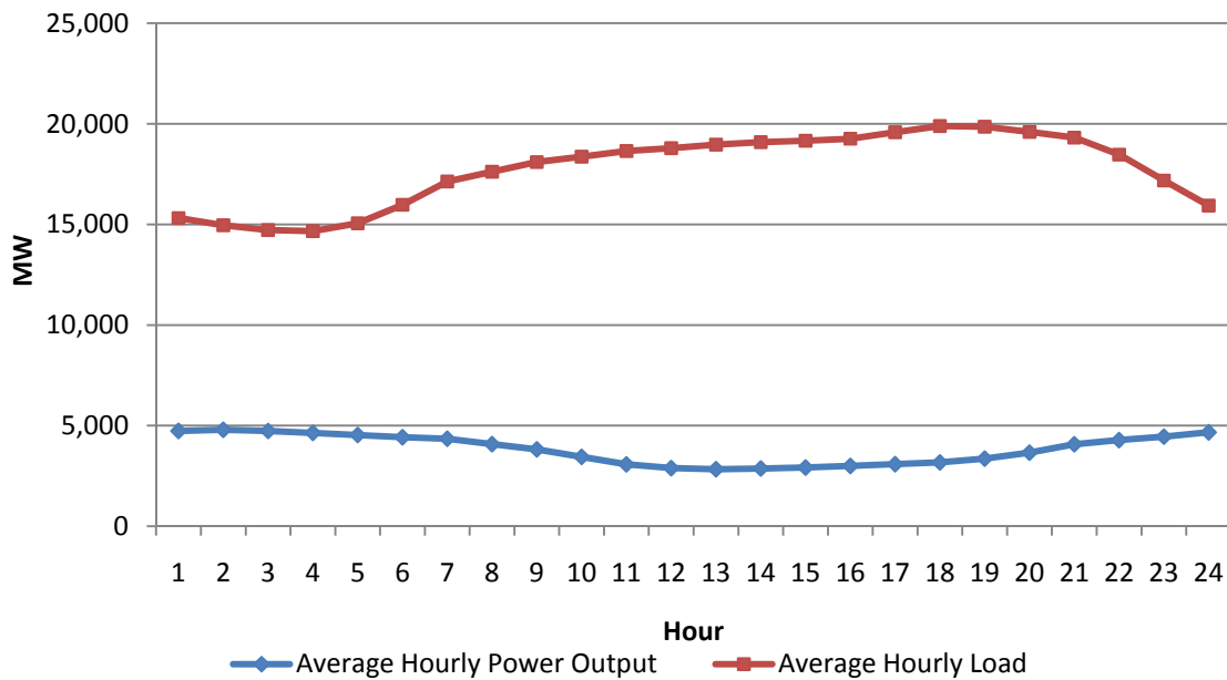
Figure 31. 1999 Mean Diurnal Coincidence for TVA and 7000 MW Wind Scenario
